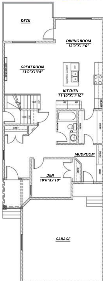
MAIN FLOOR 1064 SQ.FT.
