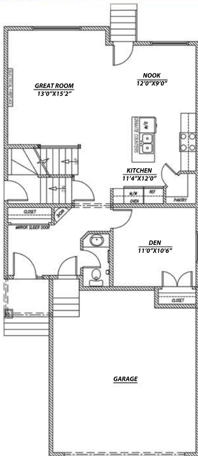
MAIN FLOOR 885 SQ.FT.
